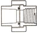
UNION COLLÉE X FILETÉE, JOINT EPDM UNION Soc Fipt with EPDM O-ring Seal
